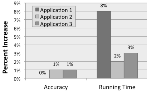
Figure 8: BraceForce’s percent increase in accuracy and running time vs. Android alone
