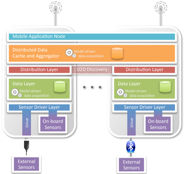
Figure 1: BraceForce: Uniform Environment
