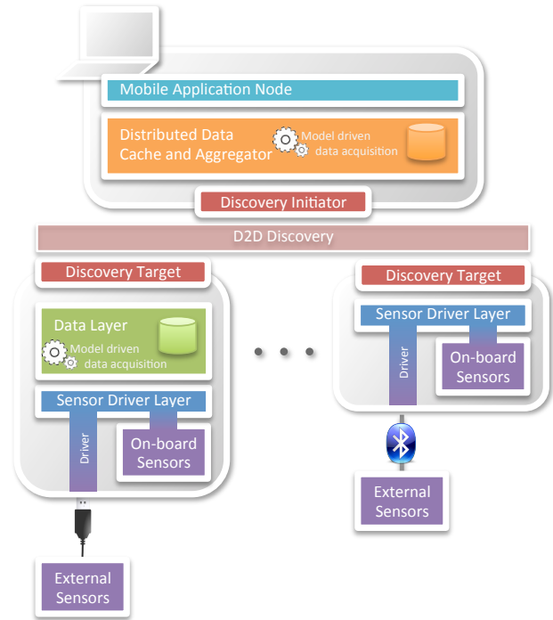
Figure 2: BraceForce: Mixed Environment
